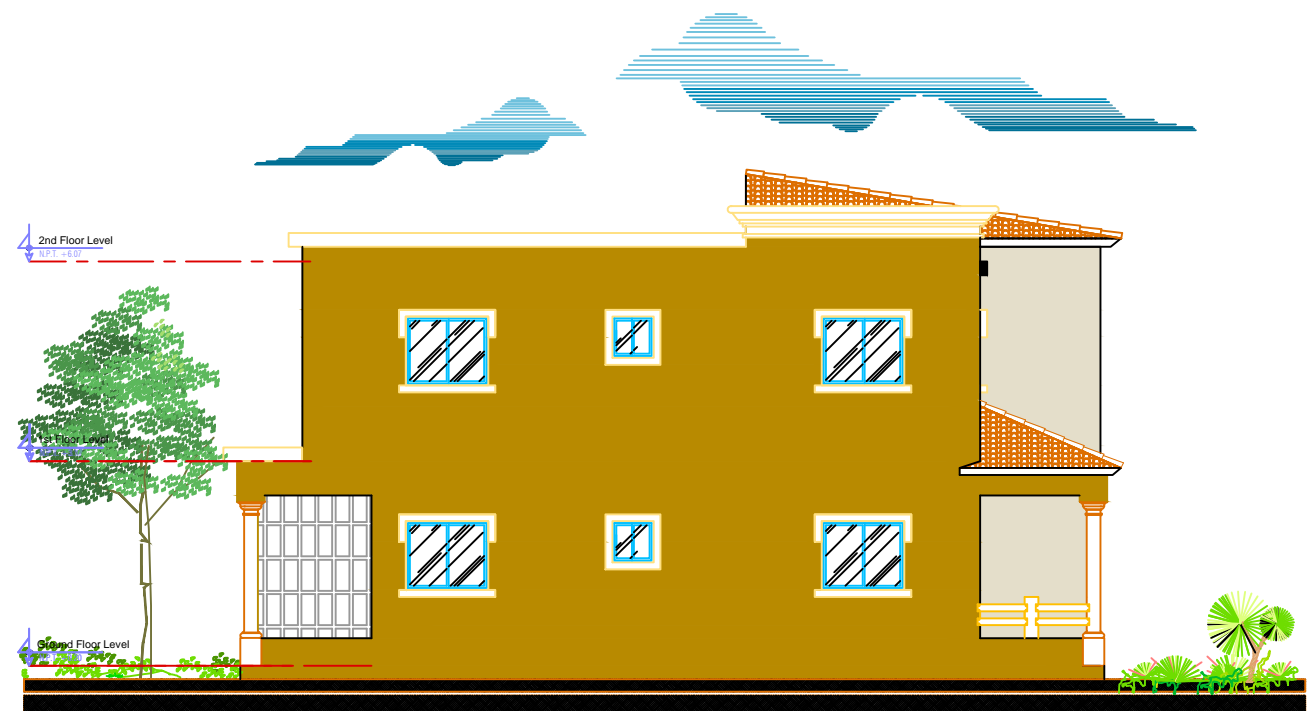
Front Lat. Left Side View F2 Building Area 171.84M 2 SCALE 1-50
