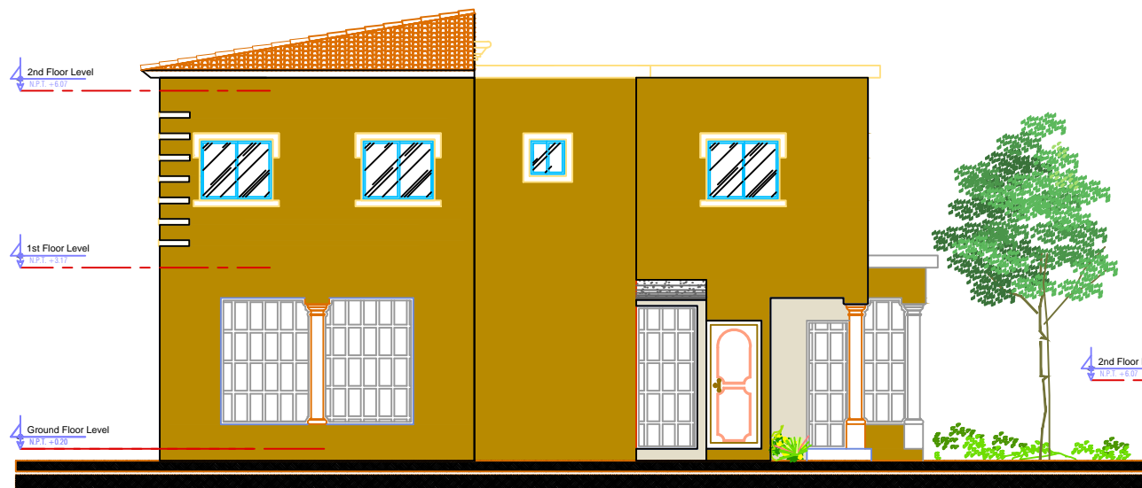
Front Lat. Right View F4 Building Area 171.84M 2 SCALE. 1-50
