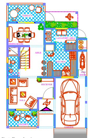
First Floor Level Building Area 84.88M 2 SCALE 1-100
