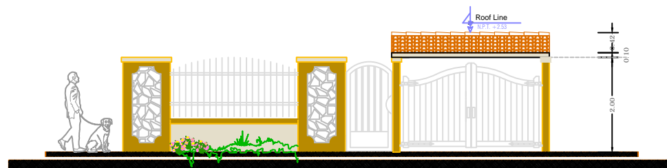
Facade Gate SCALE 1-50
