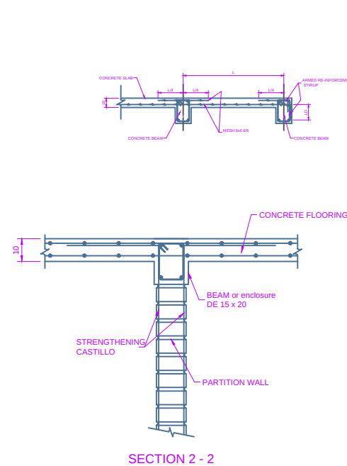
SECTION 2 - 2
