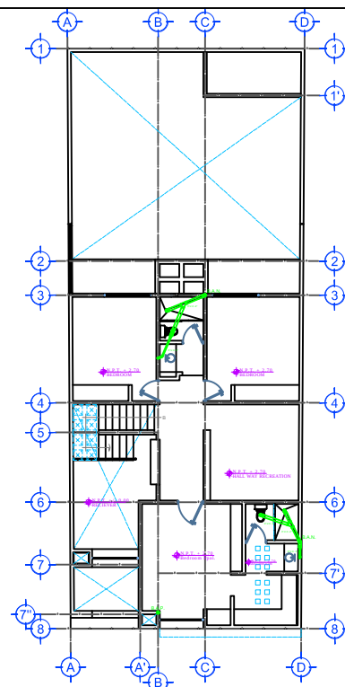
SANITARY DRAINAGE PLAN SCALE: 1:125
