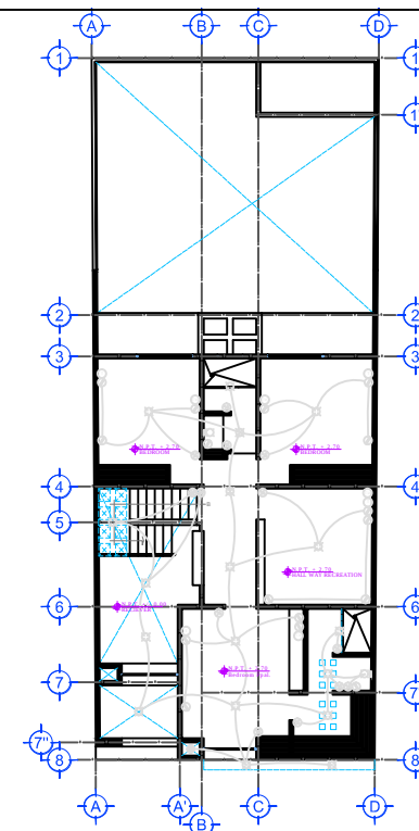
INST. ELECTRICAL FLOOR PLAN SCALE: 1:125
