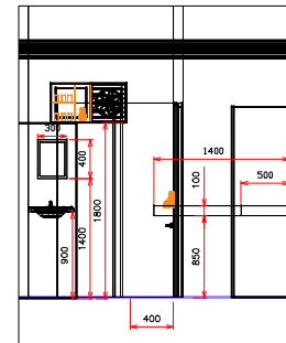
COMFORT ROOM FRONT VIEW
