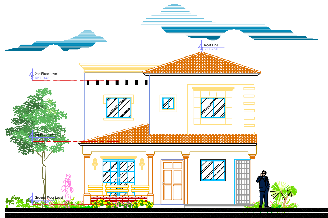
FRONT ELEVATION F1 Building Area 171.84M 2 SCALE 1-50
