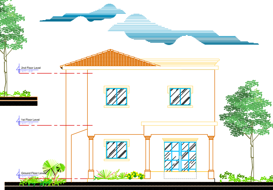
Rear Elevation F3 Building Area 171.84M 2 SCALE 1-50
