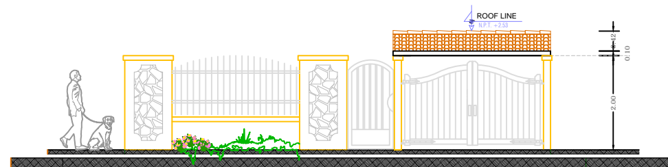
Facade Gate SCALE 1-50
