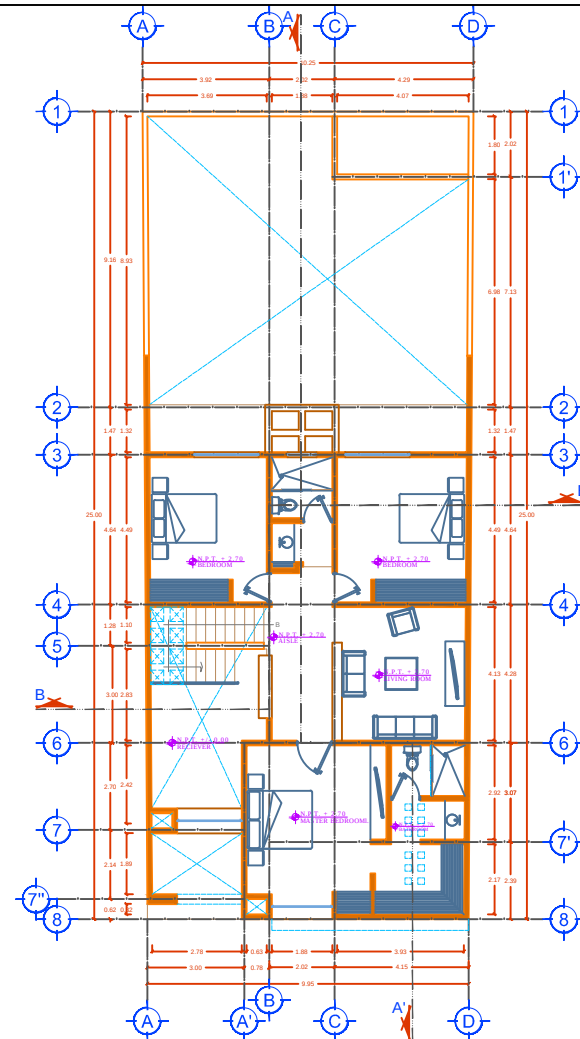
2ND FLOOR PLAN ARCHITECTURAL Scale: 1: 100
