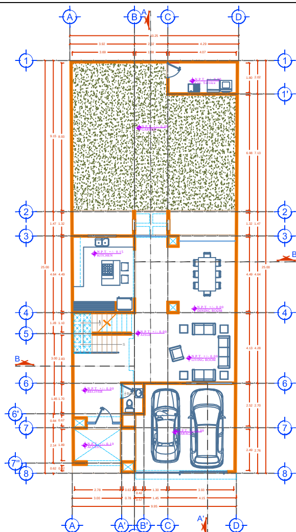
GROUND FLOOR ARCHITECTURAL Scale: 1: 100
