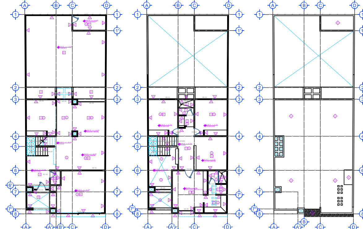
GROUND FLOOR FINISHED SCALE: 1:100
