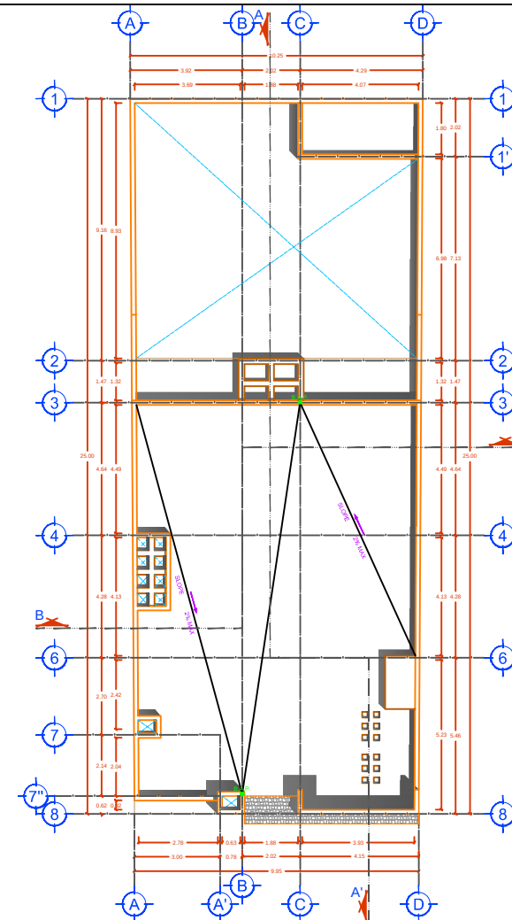
ROOF PLAN ARCHITECTURAL Scale: 1:100
