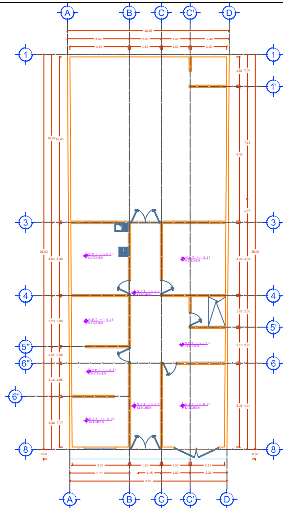
CURRENT GROUND ARCHITECTURAL Scale: 1: 100
