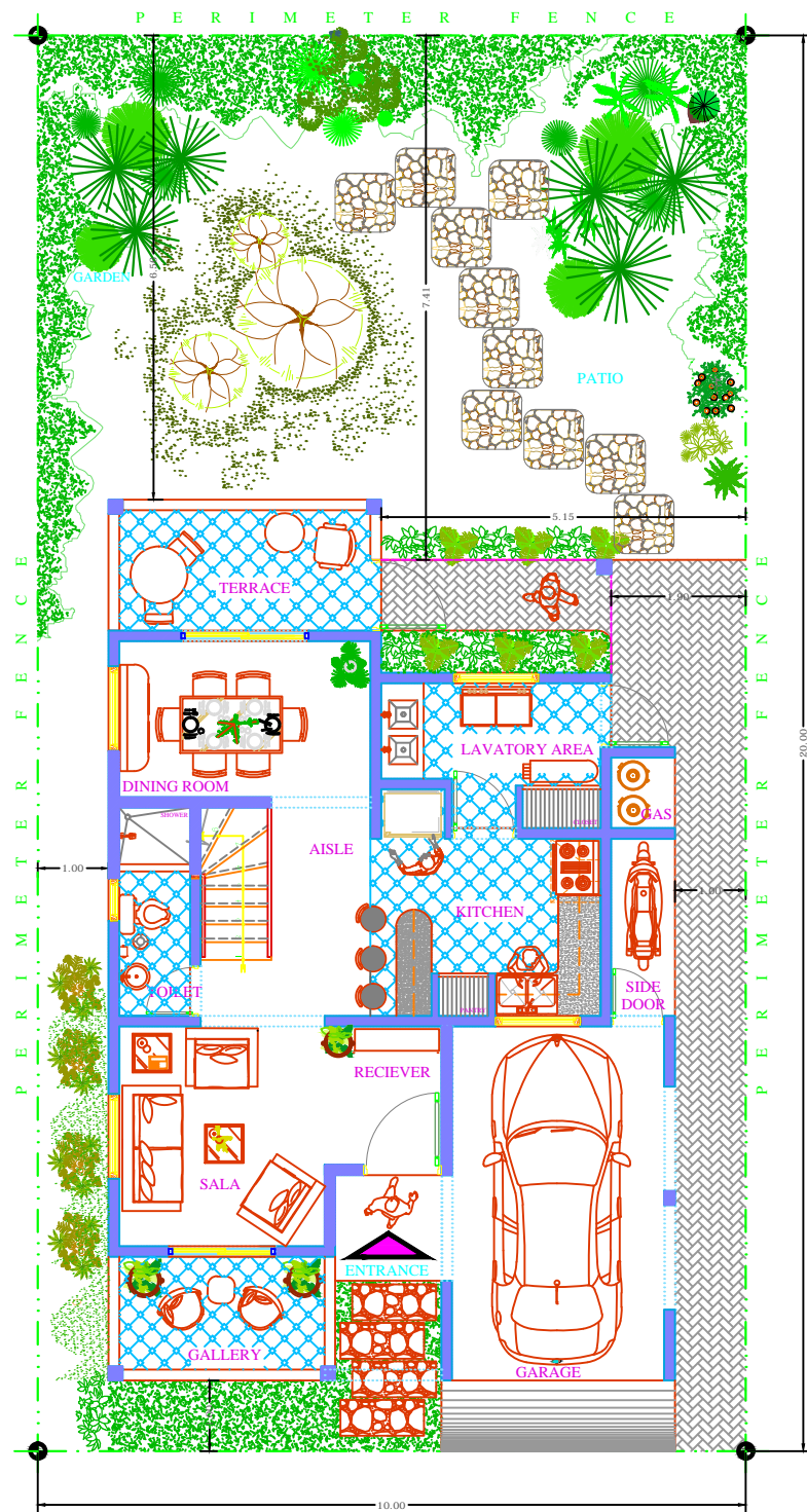
Floor Furnished, First Level Building Area 86.32M 2 SCALE 1-50
